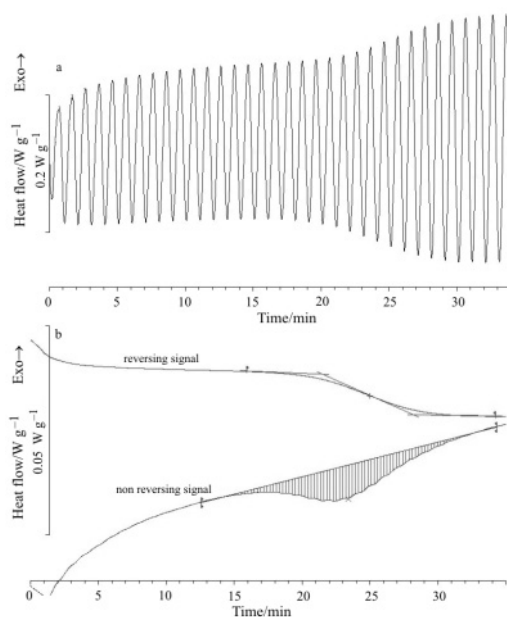
Fig. 7 a – Original modulated signal and b – transformed signal for the glass-transition of a honey sample (Lavender). Temperature range: –65 to –30°C
