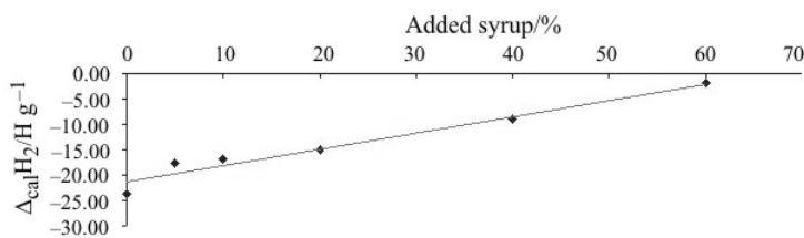
Fig. 4 Effect of added syrup on the enthalpy change of transition 2 of a pure honey
